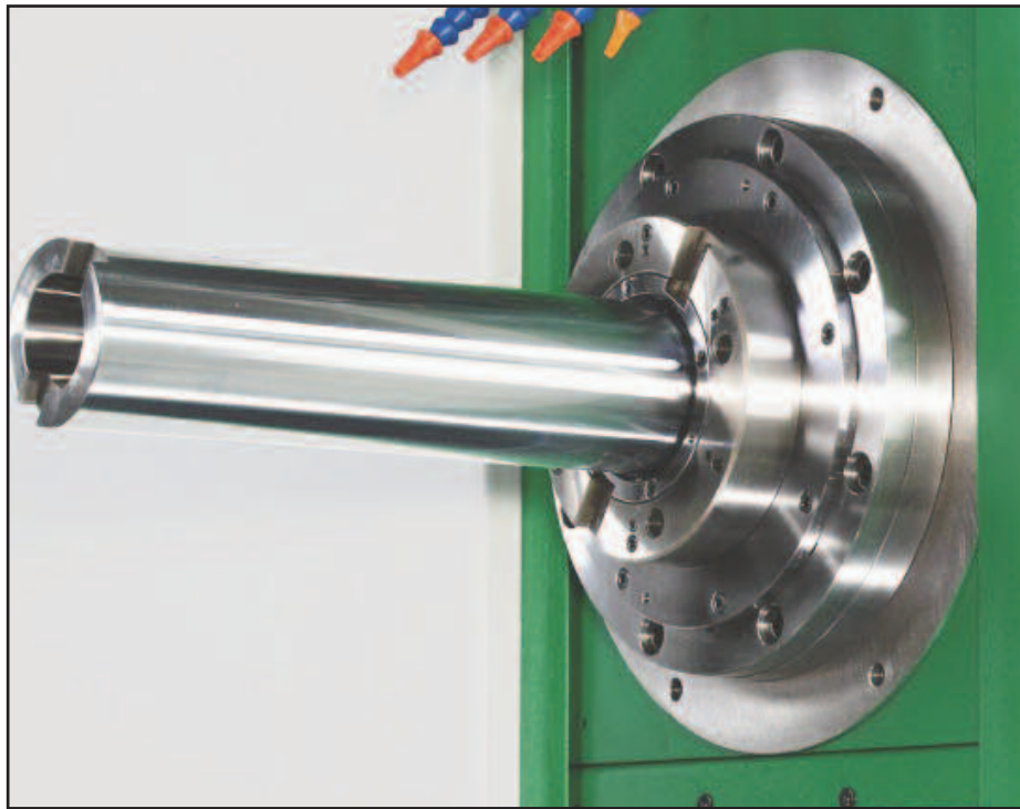
Main Spindle
