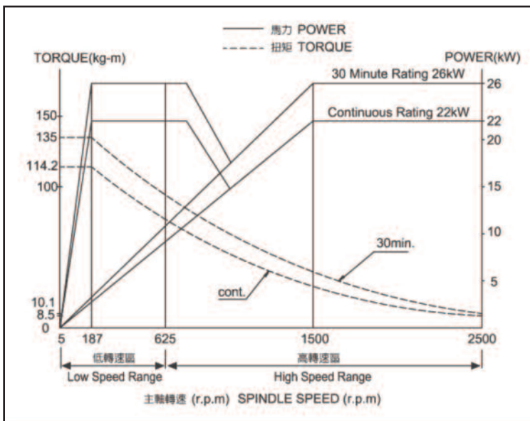
Torque Chart
